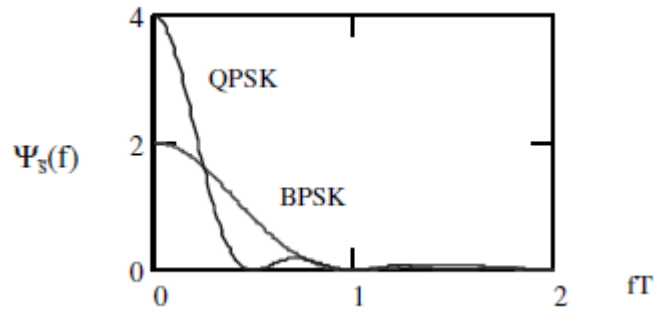
Comparison of ESD for BPSK and QPSK
