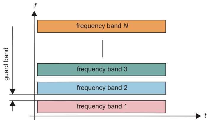
FDMA
