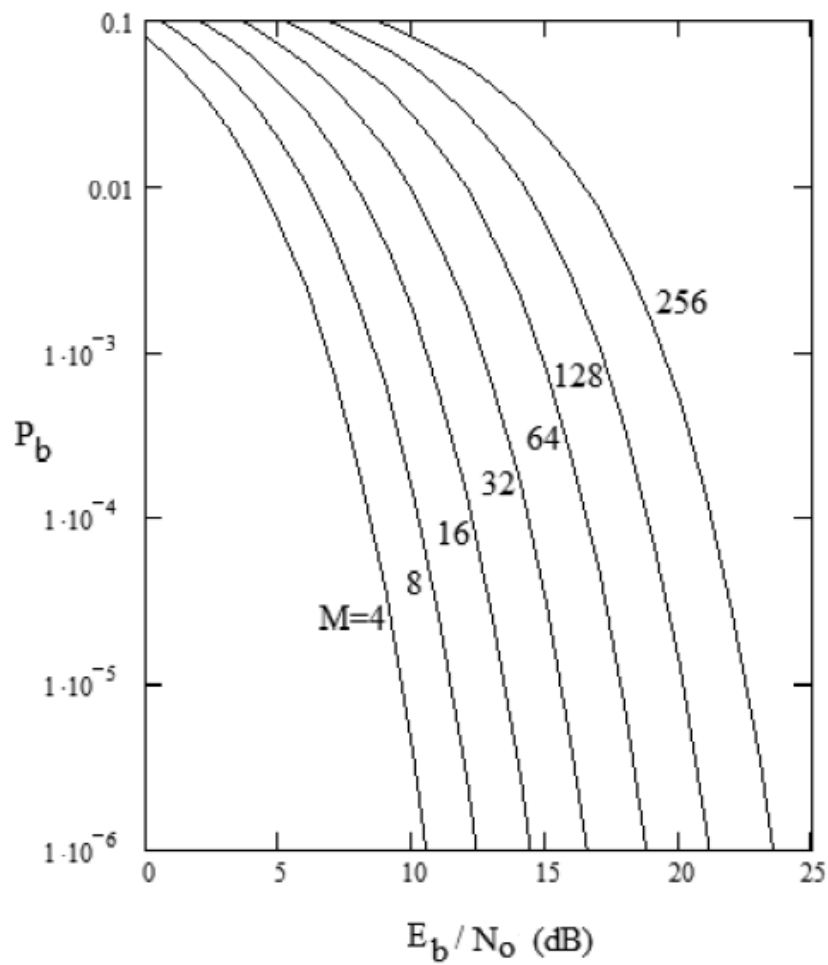
square M -QAM
